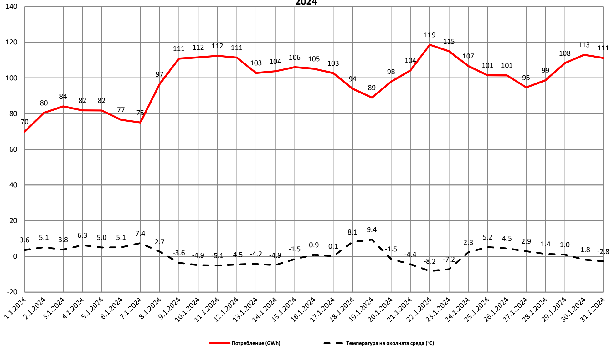
Annex 5.2 - Comparison of the gas consumption in Bulgaria and ambient temperature (Sofia) for January 2024
