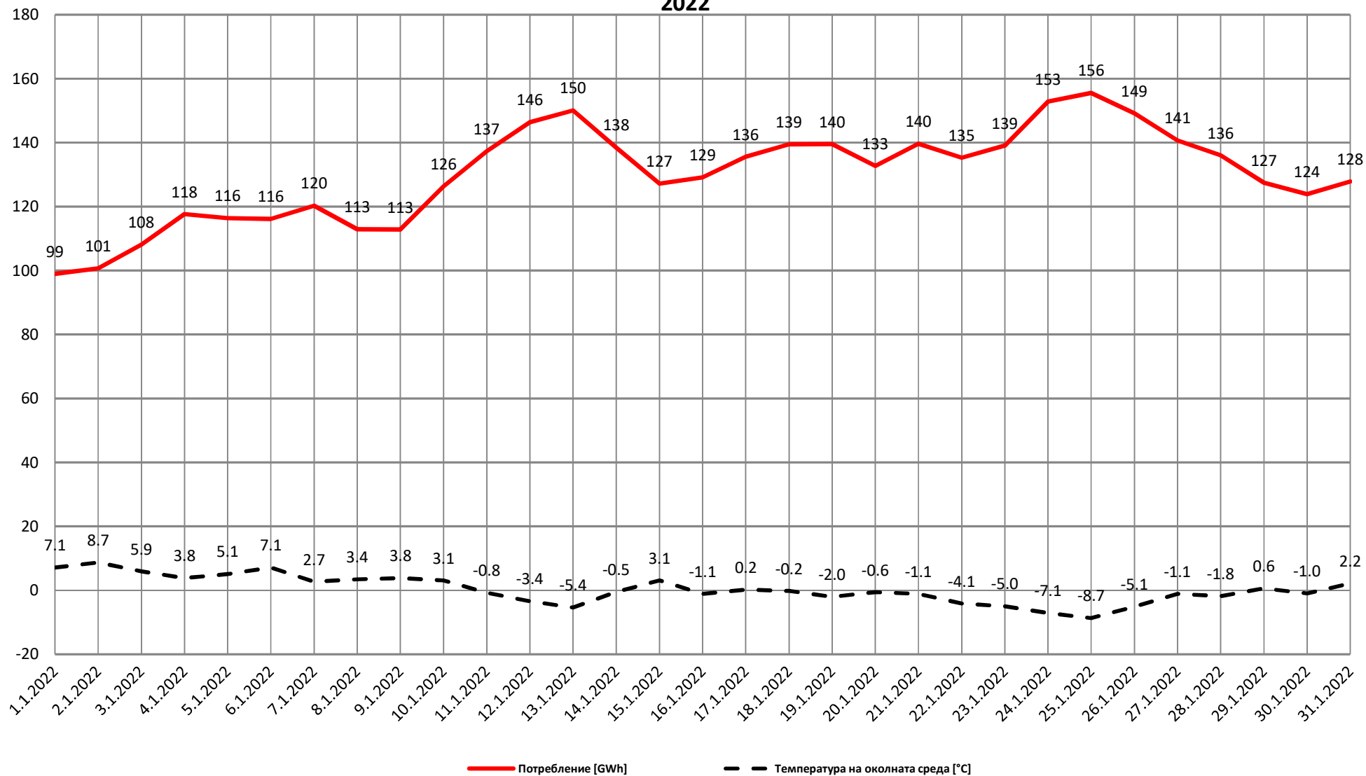
Annex 5.2 - Comparison of the gas consumption in Bulgaria and ambient temperature (Sofia) for January 2022
